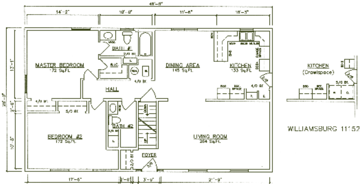
1st Floor – Williamsburg 11150 (End Kitchen - Bath & 1/2 - Basement) Series B 11152 (Crawlspace) - see inset
