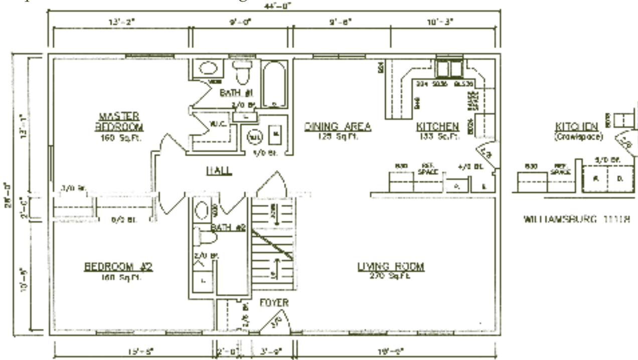
1st Floor – Williamsburg 11117 (End Kitchen - Bath & 1/2 - Basement) - Series B 11118 (Crawlspace) - see inset
