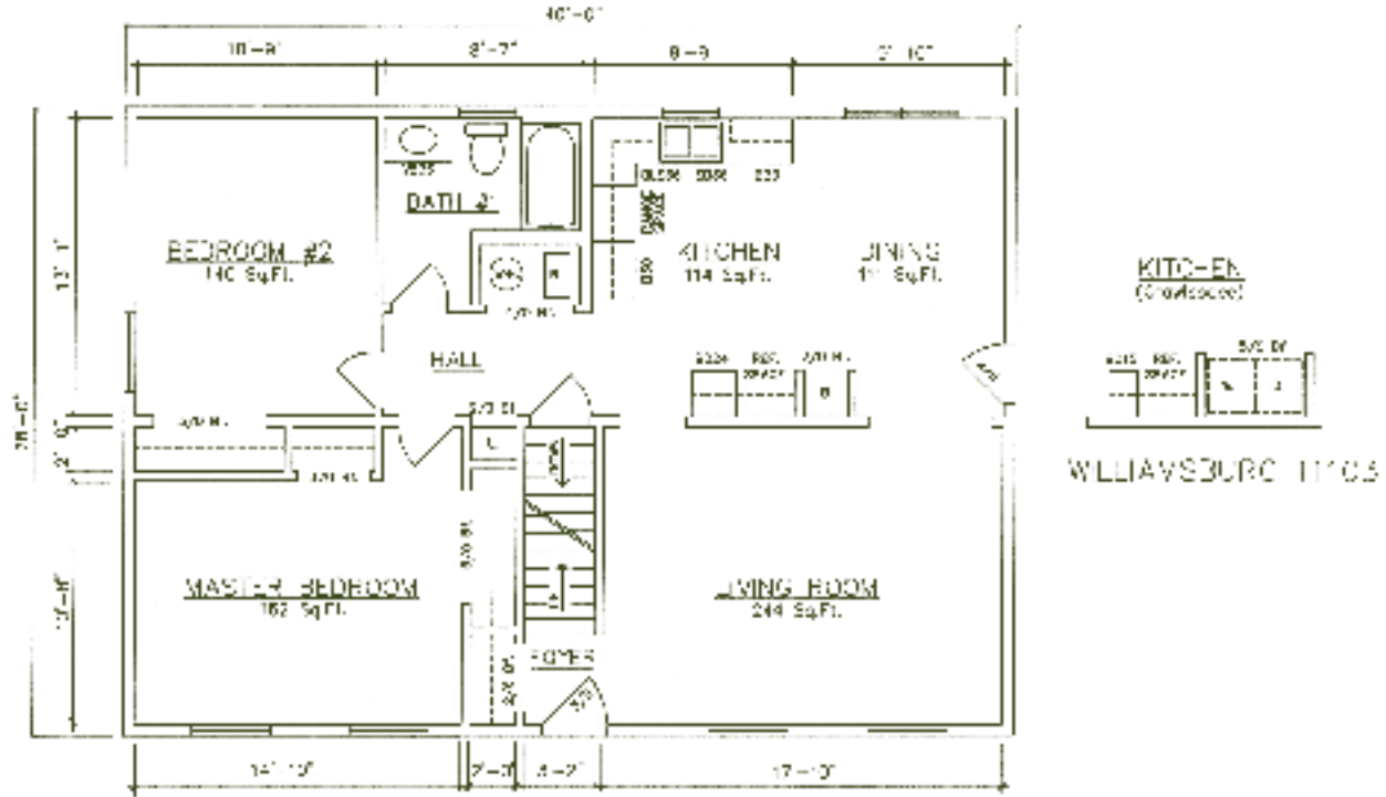
1st Floor – Williamsburg 11105 (Center Kitchen - Basement) - Series A 11103 (Crawlspace) - see inset
