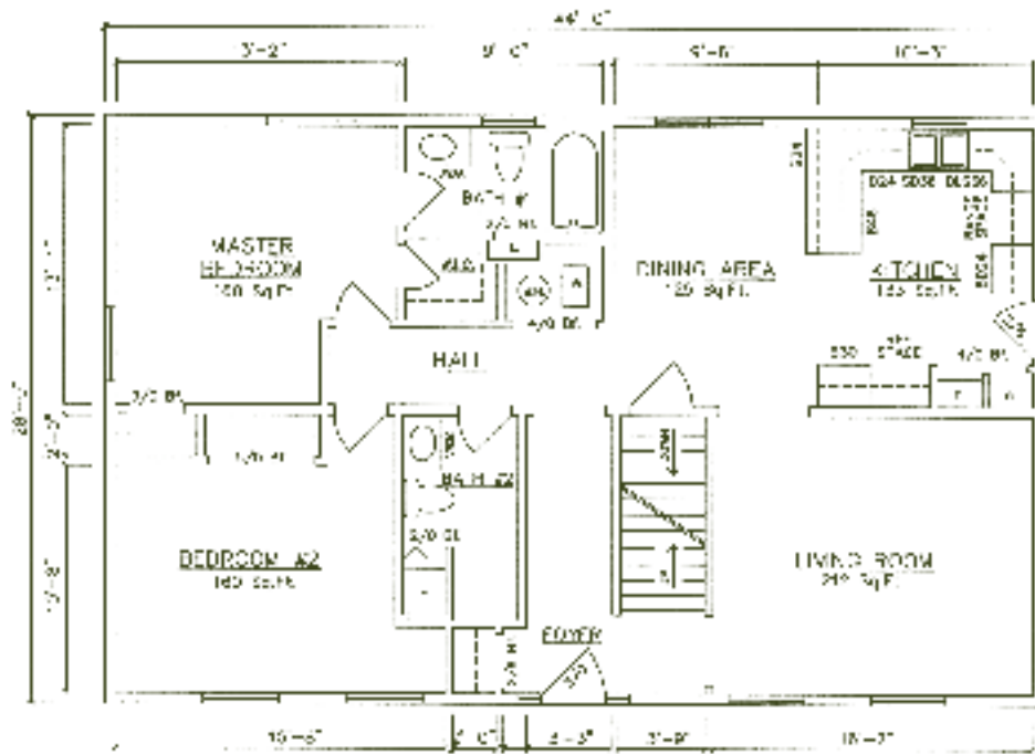
1st Floor – Williamsburg 11117 (With Center Hall Option) - Series B
