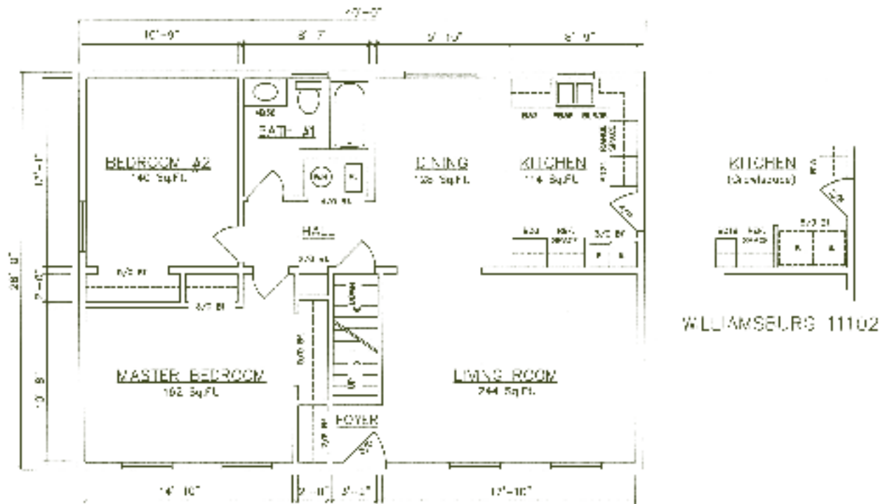
1st Floor – Williamsburg 11104 (End Kitchen - Basement) - Series A 11102 (Crawlspace) - see inset
