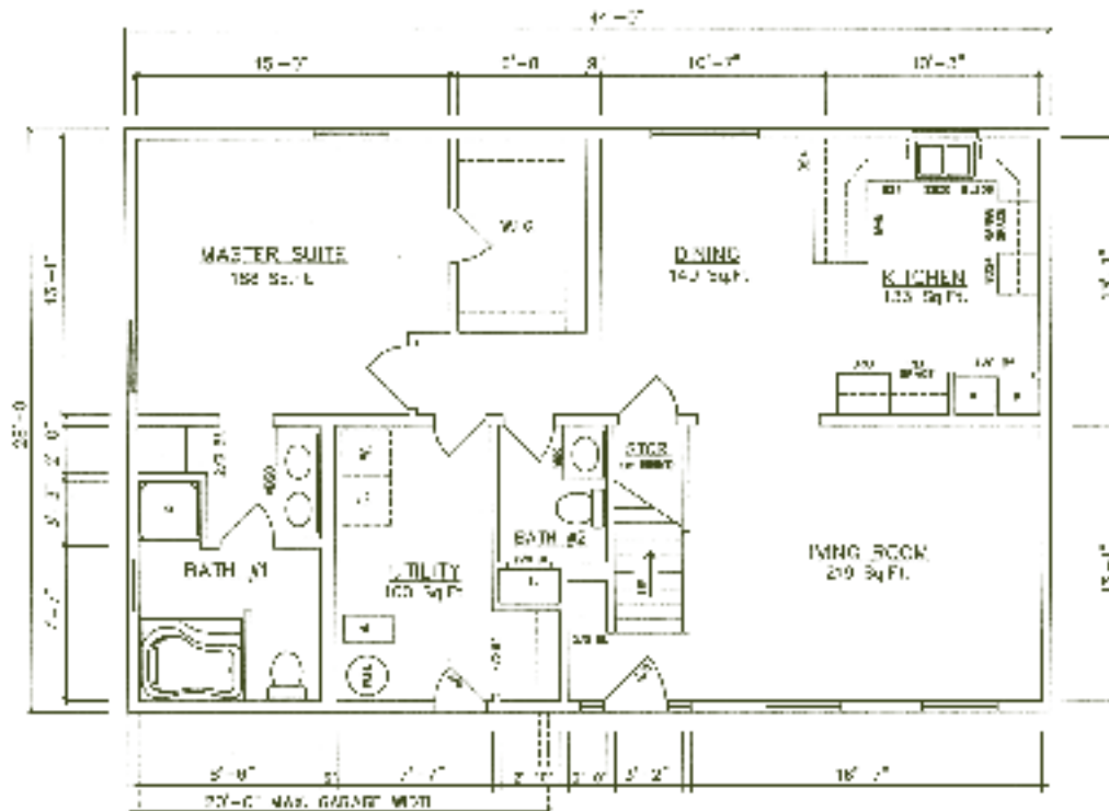
1st Floor – Williamsburg 11133 (Front Load Garage - Basement) - Series C 11137 (Front Load Garage - Crawlspace) - Series C
