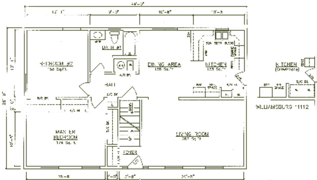
1st Floor – Williamsburg 11101 (End Kitchen - Basement) - Series A 11112 (Crawlspace) - see inset
