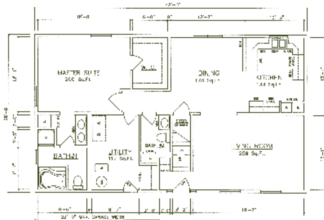
1st Floor – Williamsburg 11144 (Front Load Garage - Basement) - Series C 11146 (Front Load Garage - Crawlspace) - Series C
