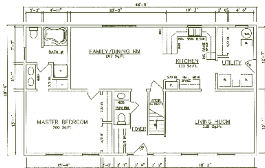
1st Floor – Williamsburg 11188 (End Utility Room - Crawlspace - R.H. - M.B.R. Suite) - Series C 11186 (Basement - Utility Room - R.H. - M.B.R. Suite) - Series C
