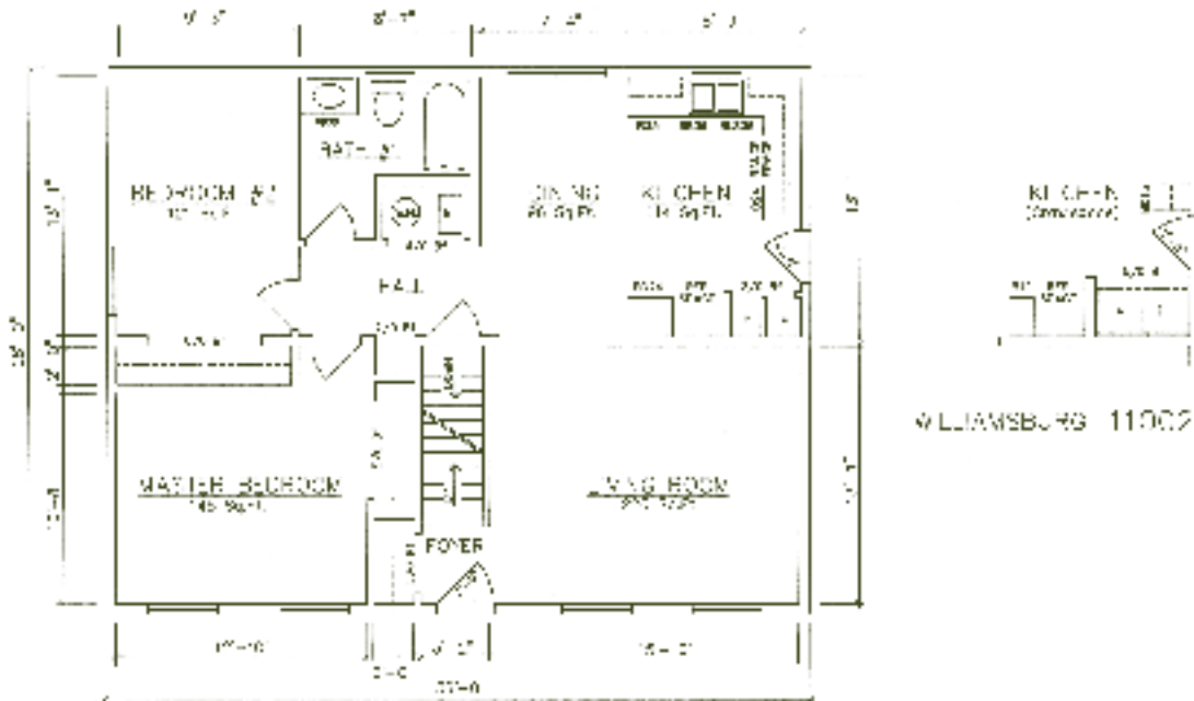
1st Floor – Williamsburg 11004 (Basement) 11002 (Crawlspace) - see inset
