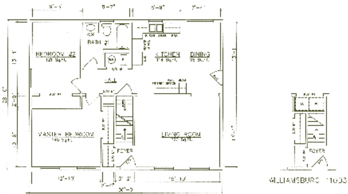
1st Floor – Williamsburg 11005 (Basement) 11003 (Crawlspace) - see inset
